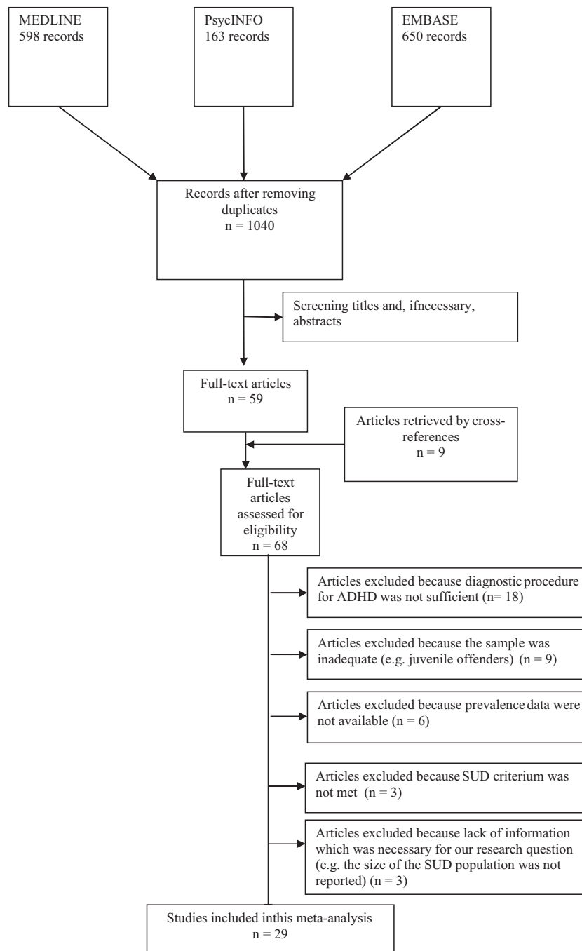
Fig. 1. Flow diagram study selection.
