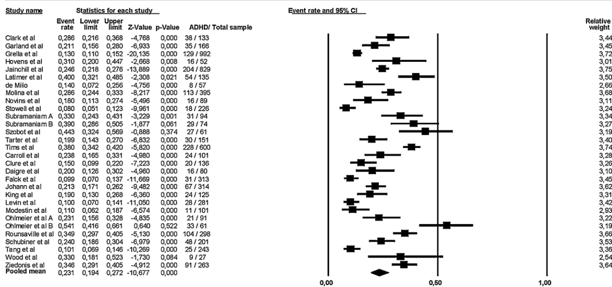
Fig. 2. Prevalence of ADHD in SUD populations. For each study ADHD prevalences (displayed as event rates), 95% confidence intervals (95% CI), numbers of ADHD cases, total sample sizes and weights are presented. At the bottom of the figure, the pooled estimate is presented.
